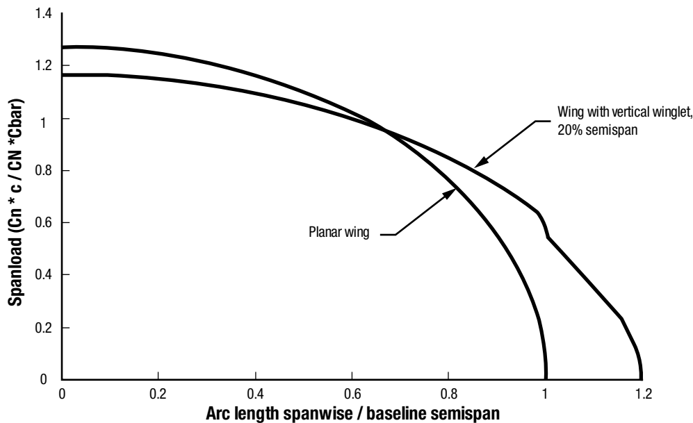
Figure 3.5. Ideal spanloads for a planar wing and a wing with a vertical winglet
