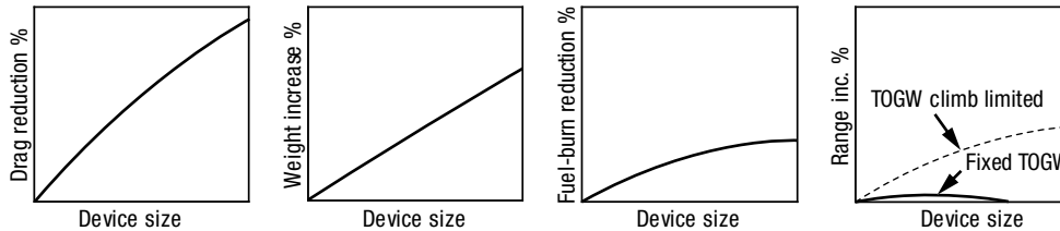
Figure 4.1 Effects of device size on performance for a generic wingtip device, assuming no excess structural margin in baseline wing
