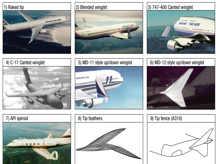
Figure 1.1. An assortment of wingtip device configurations
