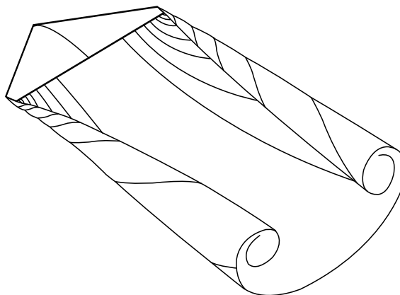
Figure 3.2. The vortex wake behind a lifting wing
