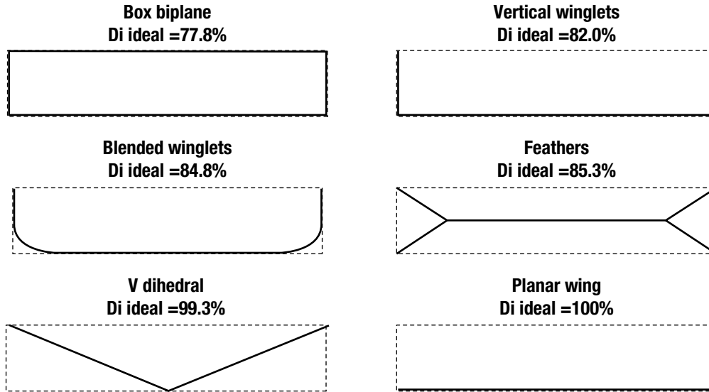
Figure 3.6. Lifting-surface configurations constrained to fit within a rectangular box in the Trefftz plane, shown in order from the lowest ideal induced drag to the highest
