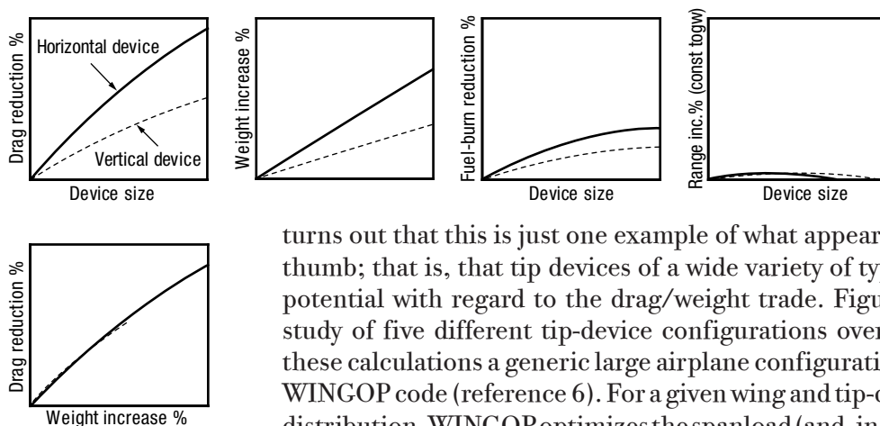
Figure 4.2. Breakdown of the drag reduction of the API blended winglets on 737NG
